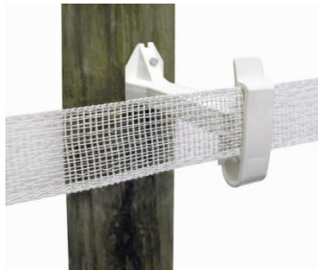
Wood Post Extender Insulator 125 mm $ 37.80 for a bag of 25 insulators
